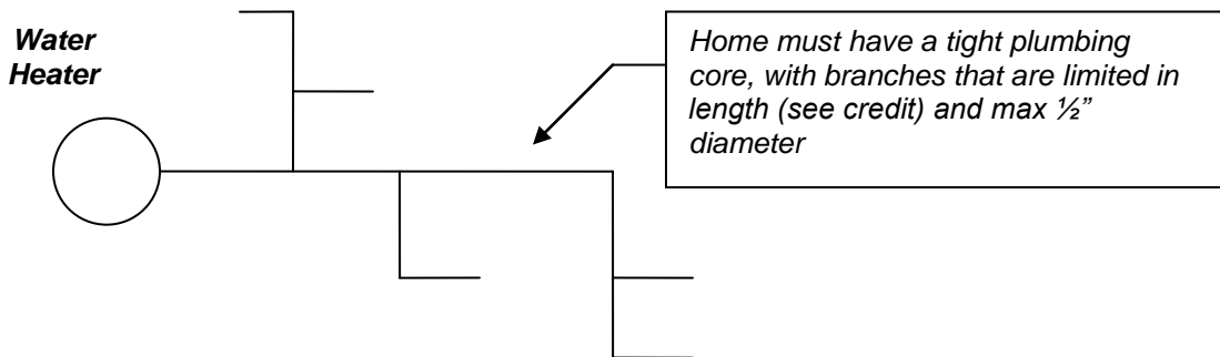
Figure 5(c). Sample Schematic of a Compact Design
